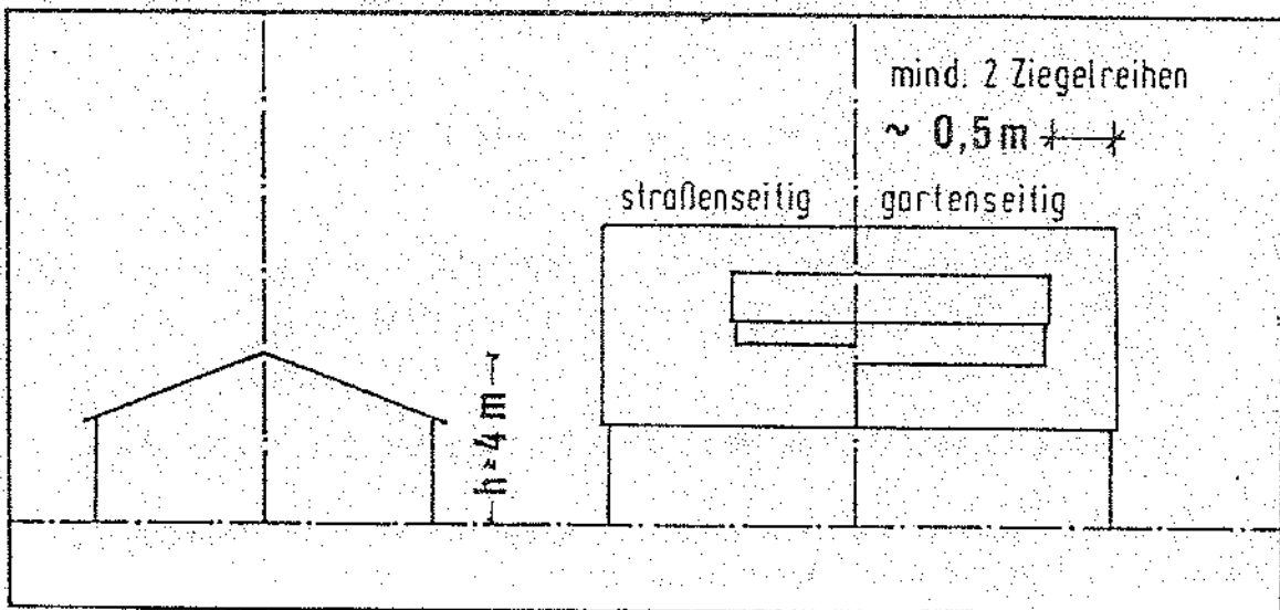
Abb. DACH:
